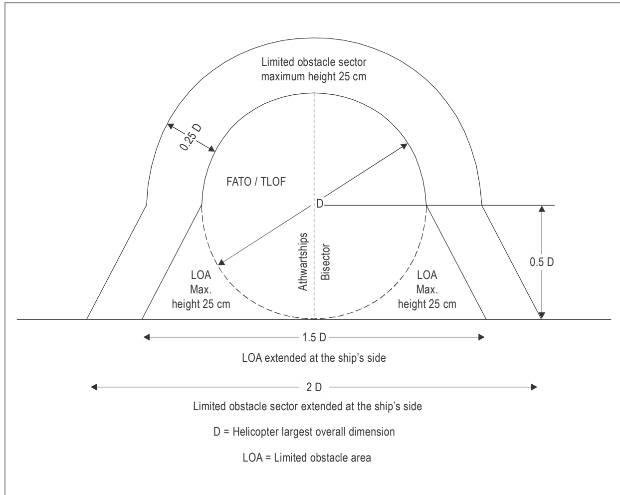
Figure I-4-2. Ships-side non-purpose-built heliport obstacle limitation sectors and surfaces
