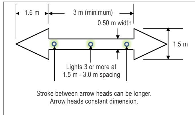
Figure II-5-20. Flight-path alignment guidance marking (dimensions)
