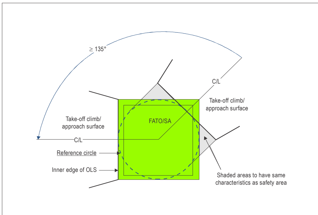
Figure II-4-2. Square FATO with reference circle and surfaces separated by 135°
