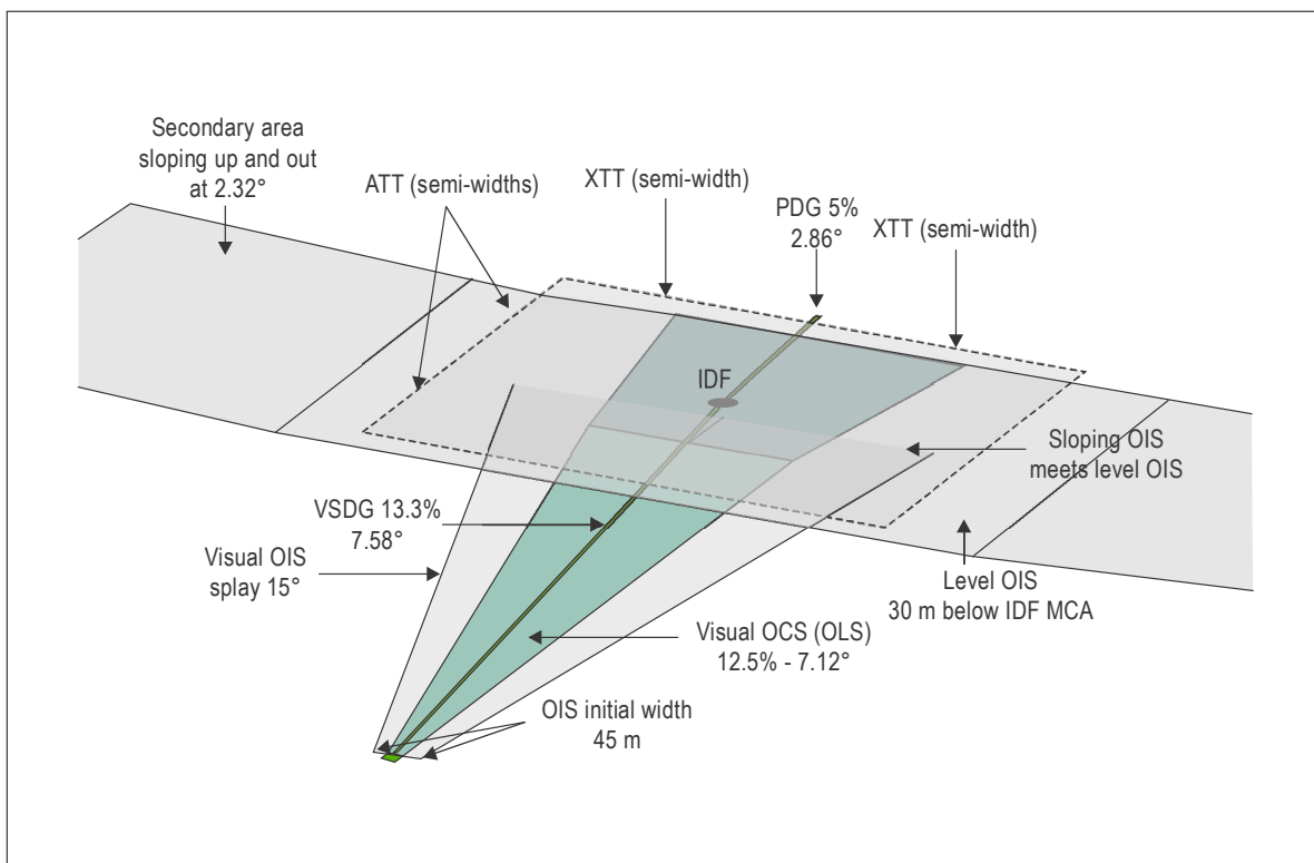
Figure 4-II-20. Direct-VS with 15 per cent divergence, 12.5 per cent gradient, IDF at 198 m (650 ft) and RNP 0.3 dimensions
