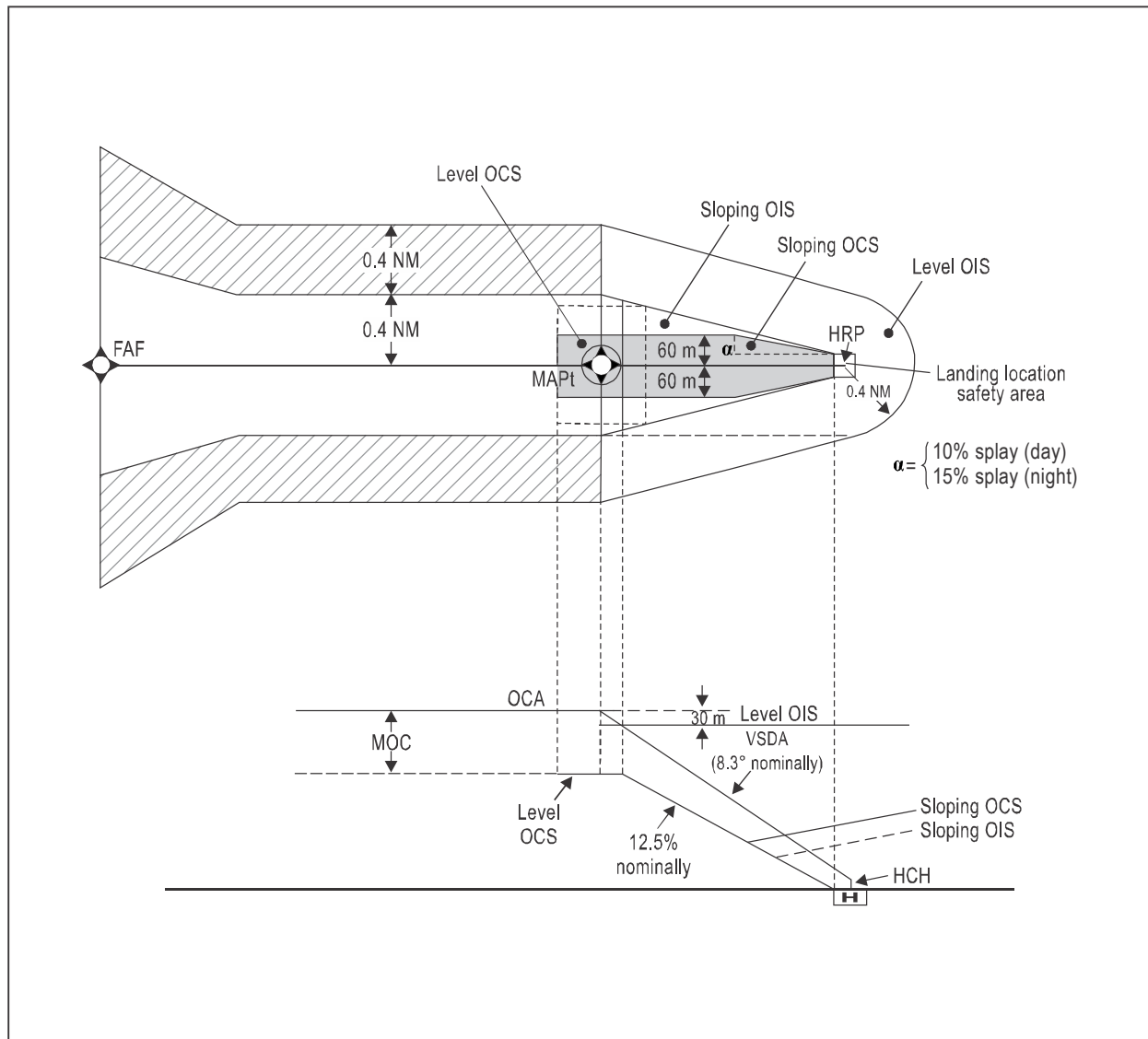
Figure II-4-14. Direct-VS (schematic)
