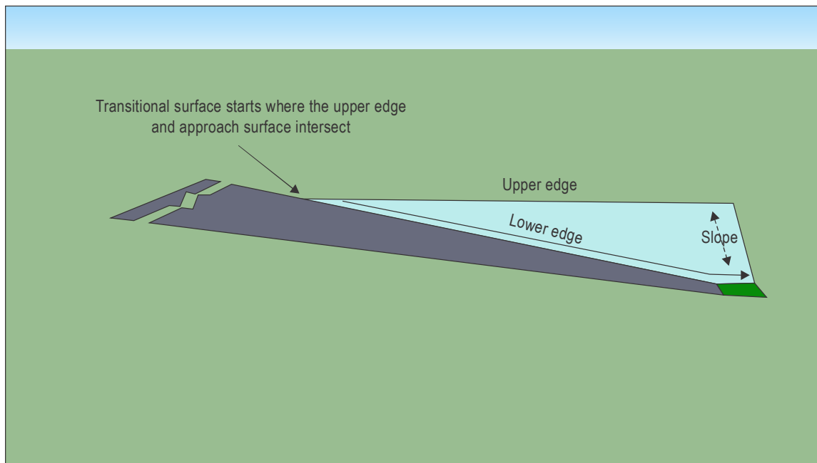
Figure II-4-7. Transitional surface
