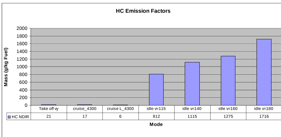
Figure 17: HC emission factors for engine idle at an indicated airspeed of 115, 140, 160 and 180 km/h (take-off and cruise for comparison and system check). HC emission factors increase drastically with increasing airspeed at engine idle. Note that the absolute scale of HC emission factors at engine flight idle may have a considerable error. (ECERT 4.4)
