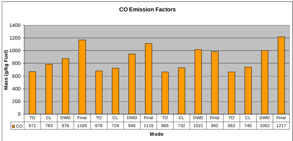
Figure 75: CO emission factors during four aerodrome circuits (TO = Take off roll, CL = Climb at v_y^6 , DWD = downwind), flown with second pilot (ECERT 62, HBKIA)
