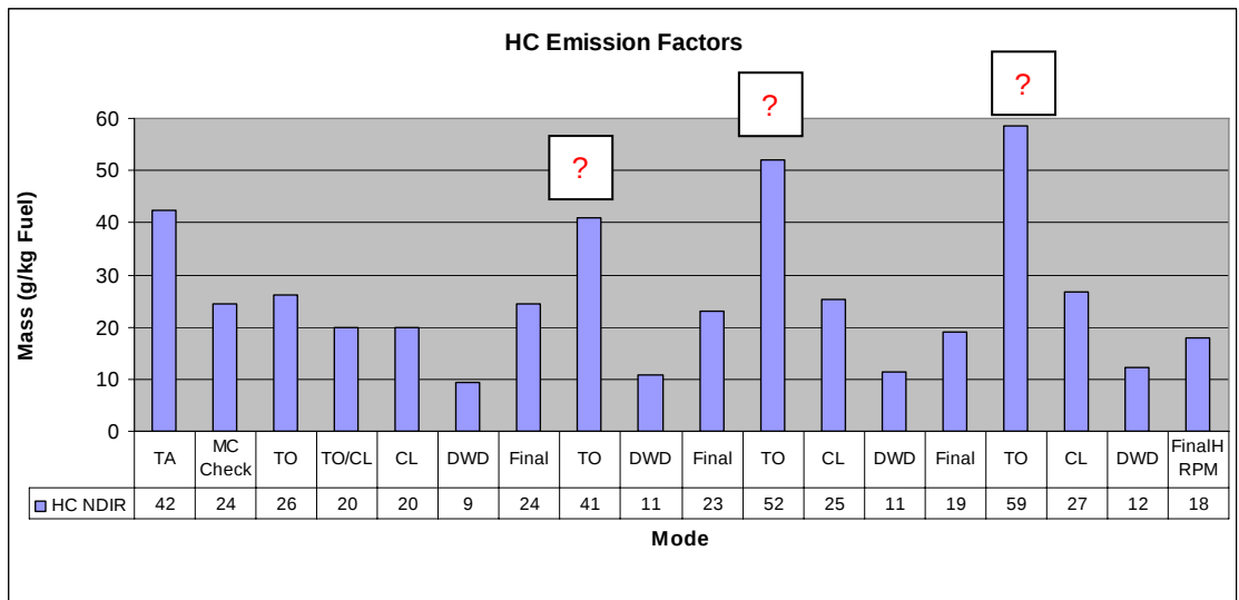
Figure 82: HC emission factors during four aerodrome circuits (TA = Taxi, MC = Magneto Check, TO = Take off roll, CL = Climb at vy, DWD = downwind), flown at Samedan Airport (ECERT 59, HBKIA)
