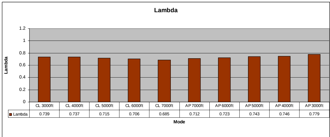
Figure 29: Change of lambda during climb at reduced power (85% engine load below 4000ft) and descent (45% engine load). All measurements with mixture “full rich”. (ECERT 11)
