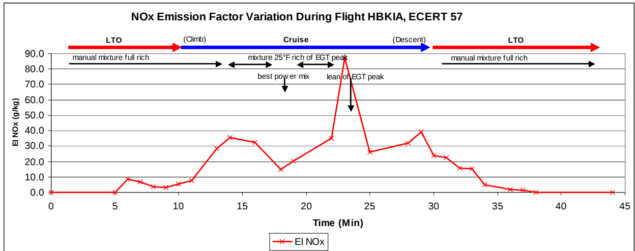
Figure 119: Variation of NO x emission factor during flight. LTO and cruise phase are indicated in red and blue darts, mixture settings in black darts. During cruise, at a mixture setting 25°F rich of peak EGT, the EI NO x is around 35 g/kg fuel. Please note, that at lean of EGT peak operation, the EI NO x would decrease below rich of EGT peak value. During this flight, this does not occur: The EGT aircraft instrumentation in HBKIA does not give individual cylinder EGT. This measurement reveals that although the mean indicated EGT value has dropped with this mixture setting, at least one of the six cylinders must have been running very hot, at peak EGT, thus producing a very high EI NO x ! (ECERT 57)
