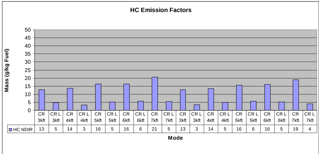
Figure 38: HC emission factors increasing with altitude without mixture adjustment. At stoichiometric mixture, the values vary around 5 g / kg fuel. In terms of typical emission measurement accuracies, the values are considered reproducible. (ECERT 9/10)
