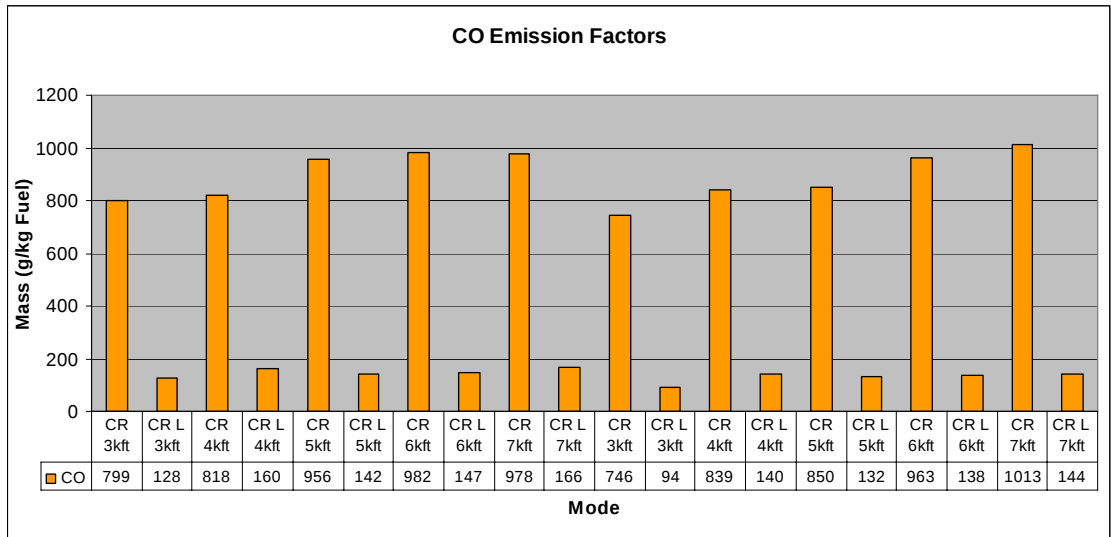
Figure 37: CO emission factors are very high and increasing with altitude without mixture adjustment. At stoichiometric mixture, the values vary around 140 g / kg fuel. In terms of typical emission measurement accuracies, the values are considered reproducible. (ECERT 9/10)
