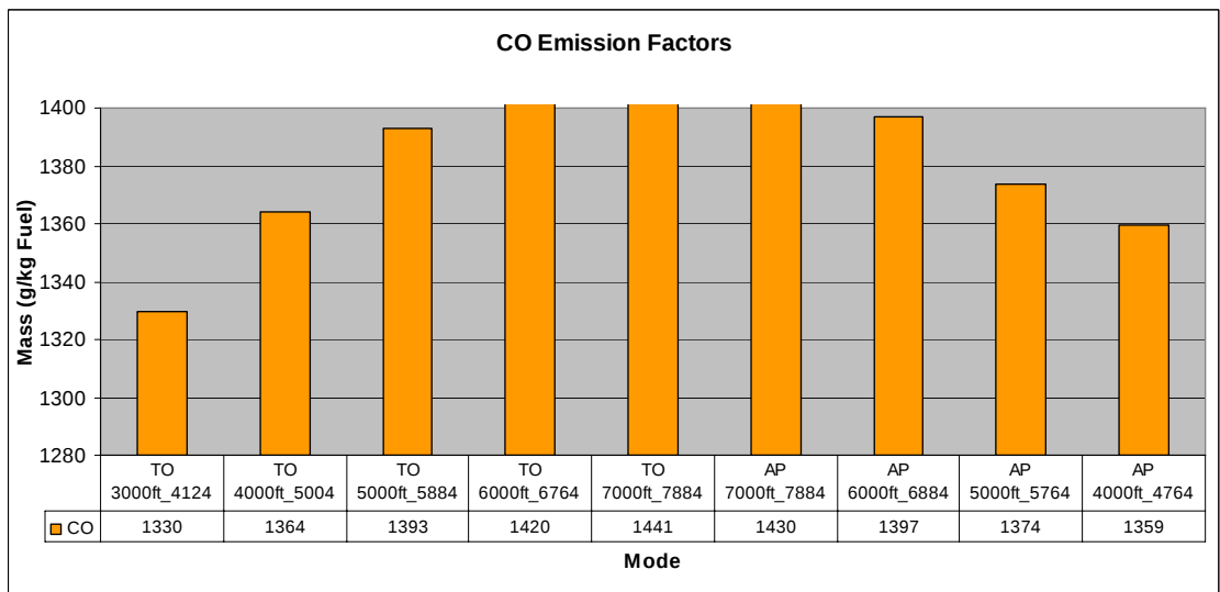
Figure 45: CO emission factors during climb at full power (TO) from 3000 to 7000ft and during descent from 7000 to 3000ft (AP). The second number after aircraft altitude in feet is the density altitude. (ECERT27, HBKEZ)
