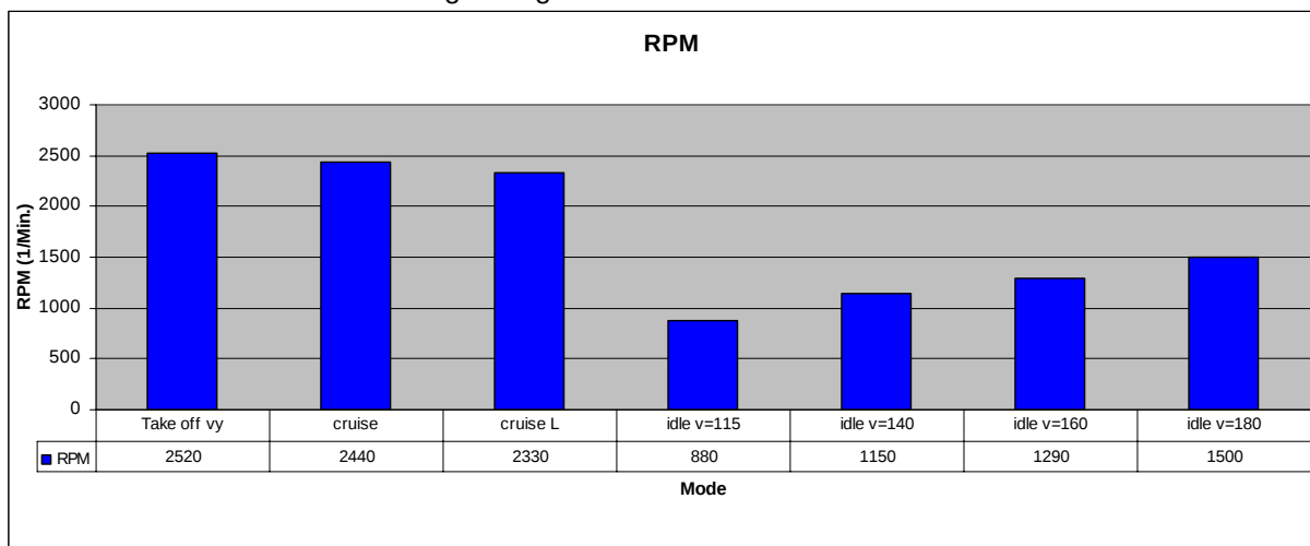
Figure 16: Engine RPM (Revolutions per Minute) at take-off and cruise (for comparison) and with engine idle at an indicated airspeed of 115, 140, 160 and 180 km/h. Idle RPM increases with increasing airspeed. (ECERT 4.4)
