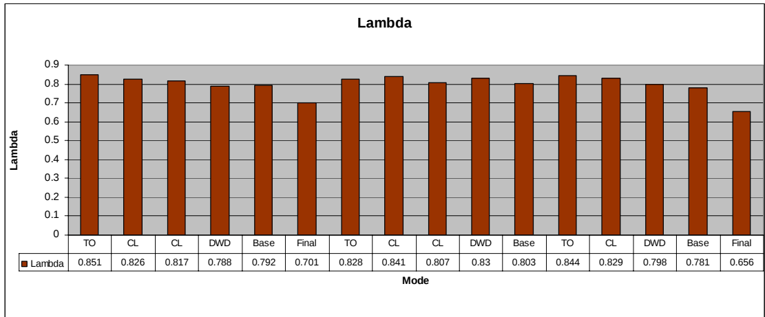
Figure 74: Lambda during three aerodrome circuits (TO = Take off roll, CL = Climb at v_y , DWD = downwind). No “Final” measurement at the second circuit. (ECERT 56, HBKIA)
