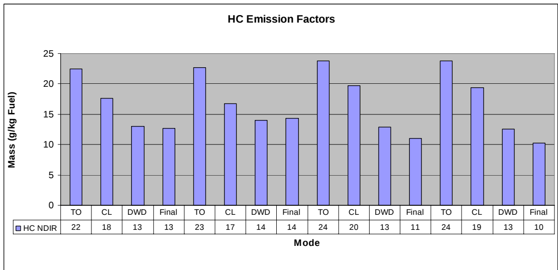
Figure 76: HC emission factors during four aerodrome circuits (TO = Take off roll, CL = Climb at v_y , DWD = downwind), flown with second pilot (ECERT 62, HBKIA)
