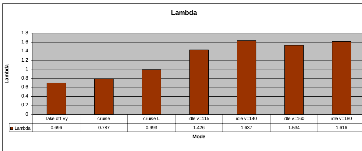
Figure 18: Lambda for engine idle at an indicated airspeed of 115, 140, 160 and 180 km/h (take-off and cruise for comparison and system check). Lambda increases far above 1 at engine flight idle condition, which shows the presence of excess oxygen in the combustion chambers of the engine, producing very lean conditions. (ECERT 4.4)
