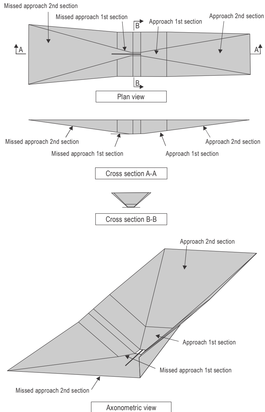
Figure 4-6. Surface for precision approaches
