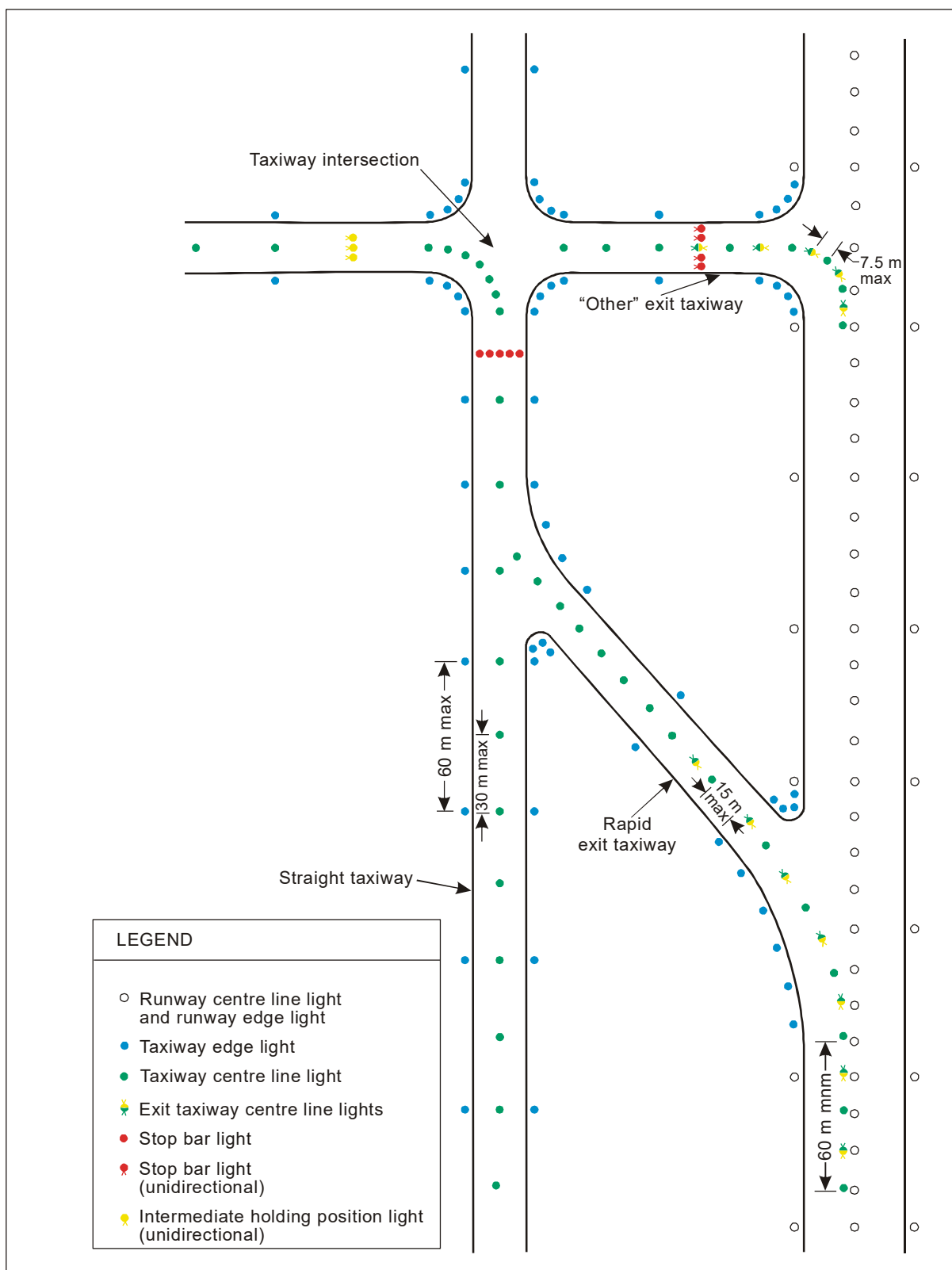
Figure 5-26. Taxiway lighting
