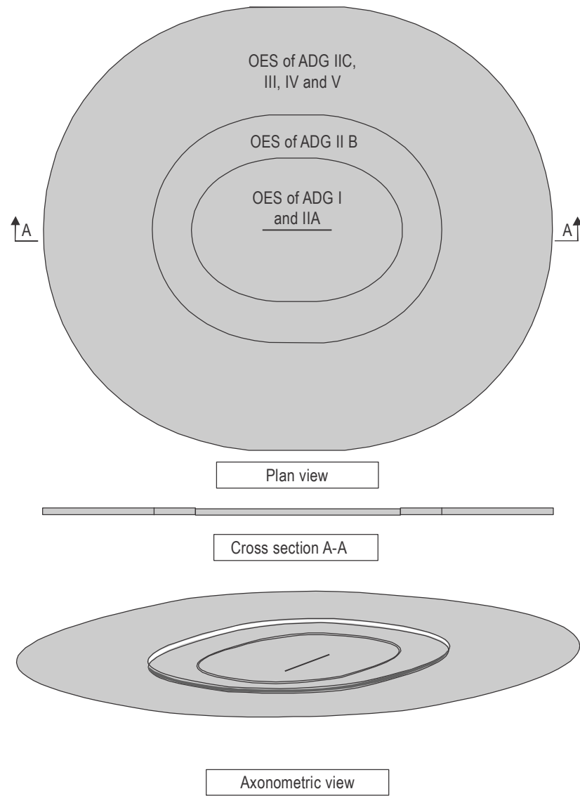
Figure 4-4. Horizontal surface
