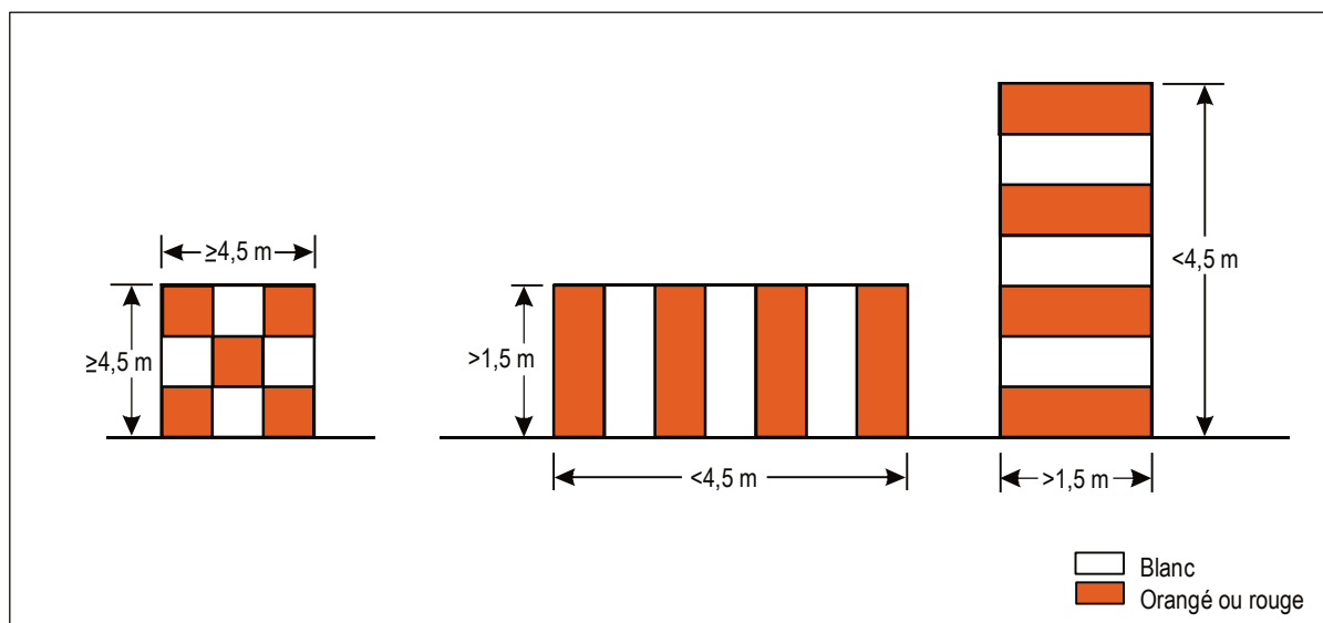
Figure 6-1. Marquages types
