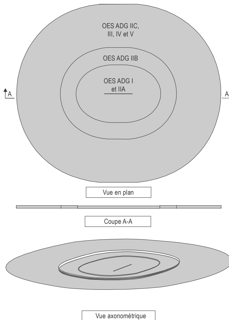
Figure 4-4. Surface horizontale
