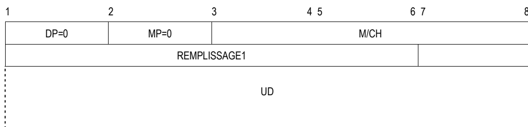
Figure 5-21. Paquet MSP COURT
