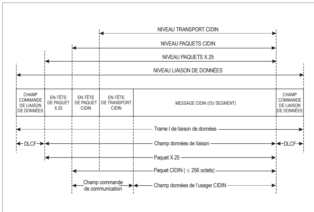
Figure 8-2. Terminologie CIDIN
