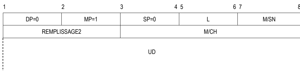
Figure 5-22. Paquet MSP LONG
